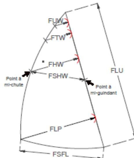
GENOIS VOLANT
